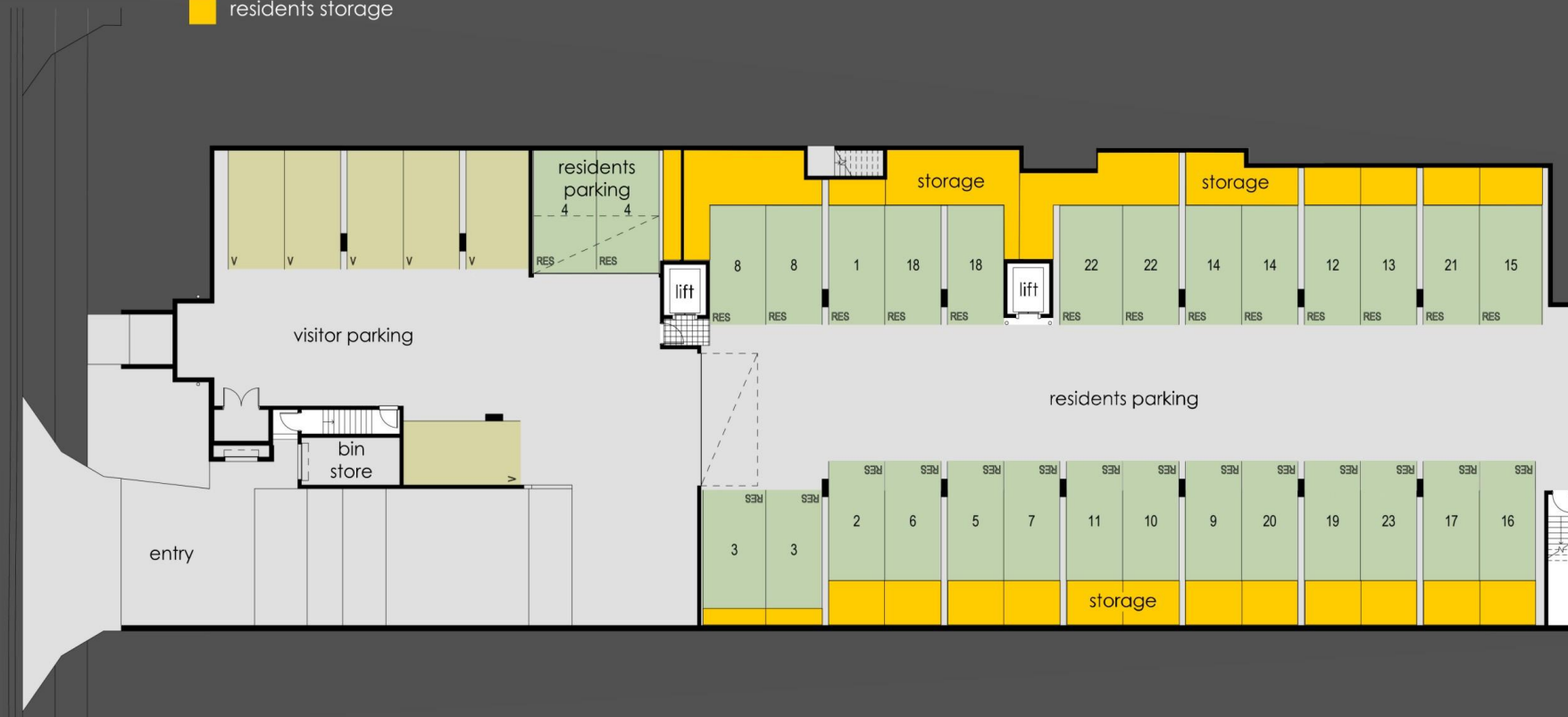
BASEMENT LEVEL PLAN
